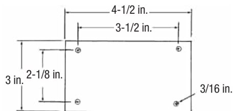
P 64 GFCI
